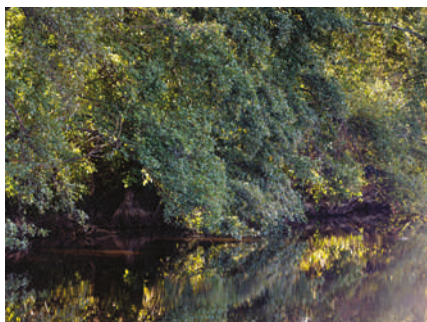
Playa fluvial Vale Juncal Vale Juncal
